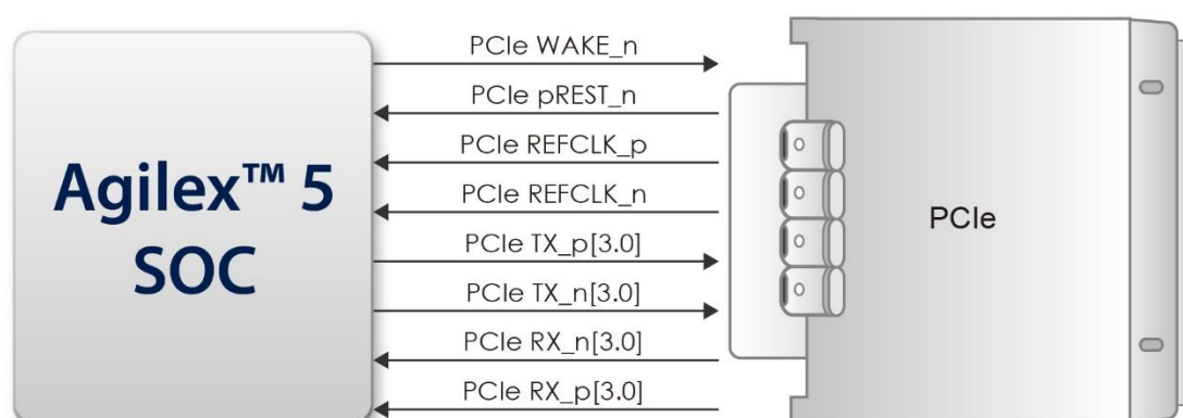
Figure 2-30 PCI Express Pin Connection
