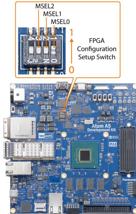
Figure 5-2 SW4 for FPGA Configuration Mode
