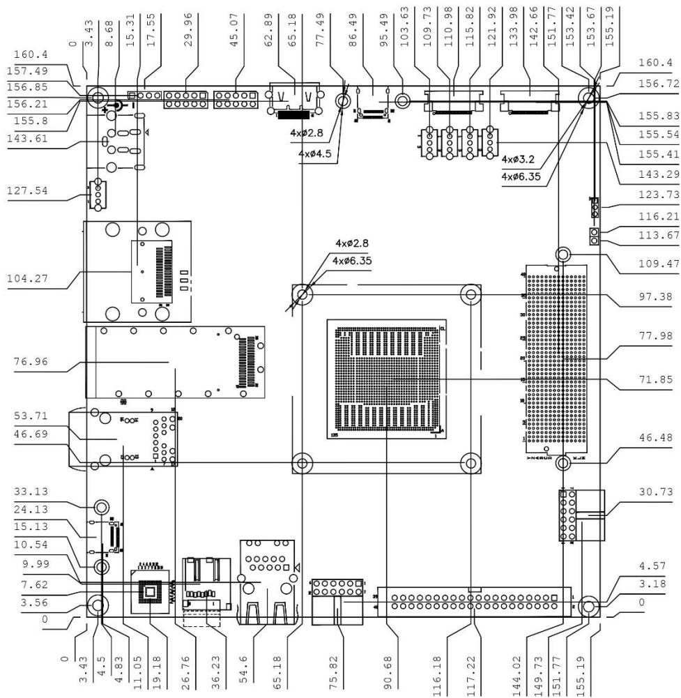
Figure 1-4 Mechanical layout
