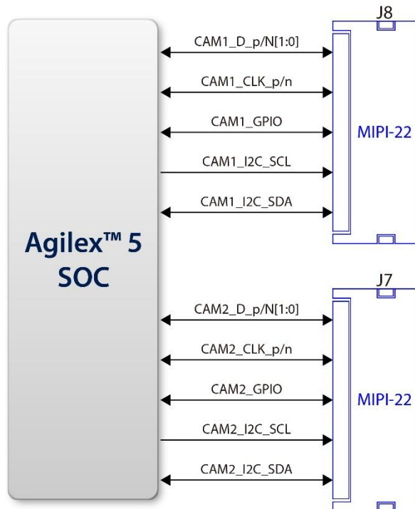
Figure 2-29 Connection between the MIPI connector and FPGA
