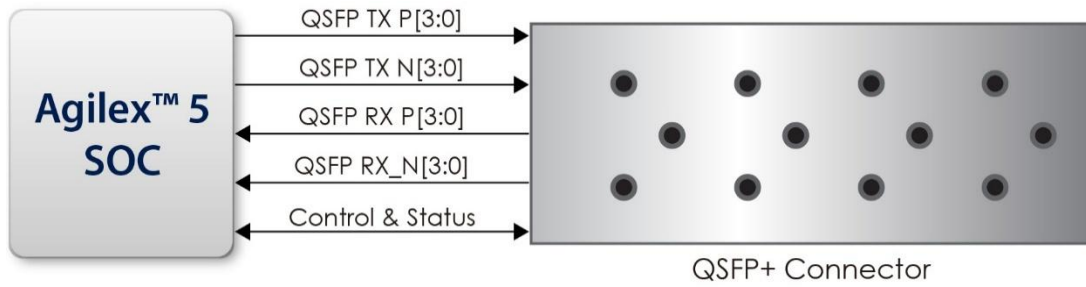
Figure 2-26 Connection between the QSFP+ and FPGA
