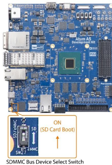
Figure 2-16 SDMMC Bus Device Select Switch
