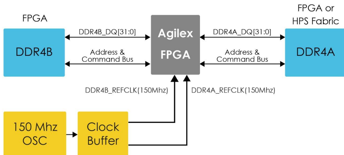
Figure 2-21 Connection between the DDR4 and Agilex 5 FPGA
