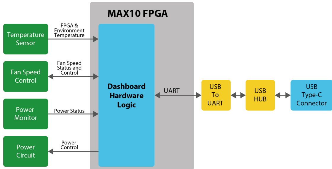
Figure 2-20 Block diagram of the system status interface
