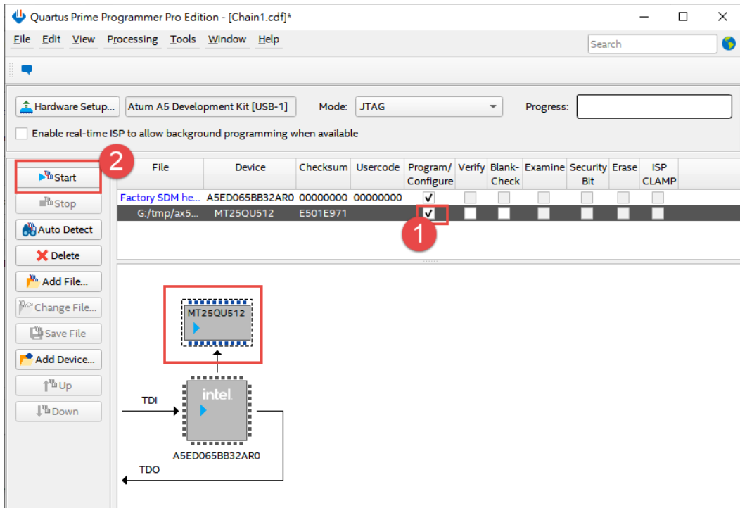
Figure 5-16 Enable programming file
