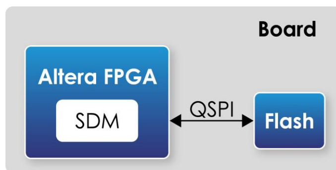
Figure 2-2 AS mode for the Atum A5 board
