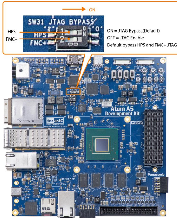
Figure 2-6 Position of slide switches SW31
