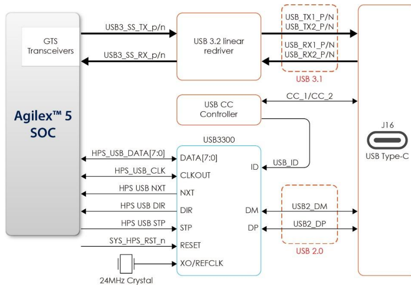
Figure 2-22 Connections between the Atum A5 and USB interface
