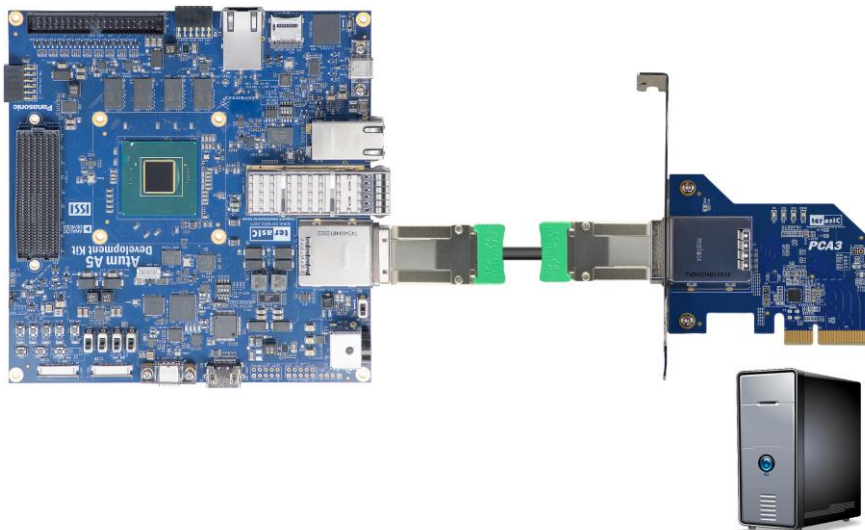
Figure 2-33 PCIe Link Setup between Atum A5 and PC
