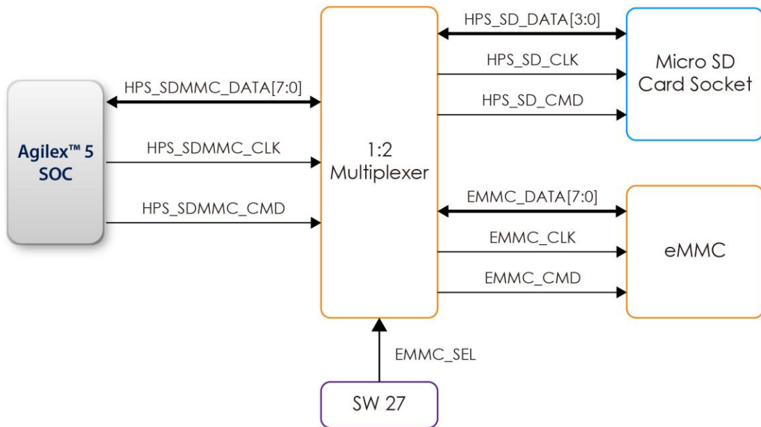
Figure 2-15 Connections between Micro SD card socket, eMMC and Agilex 5 SoC FPGA
