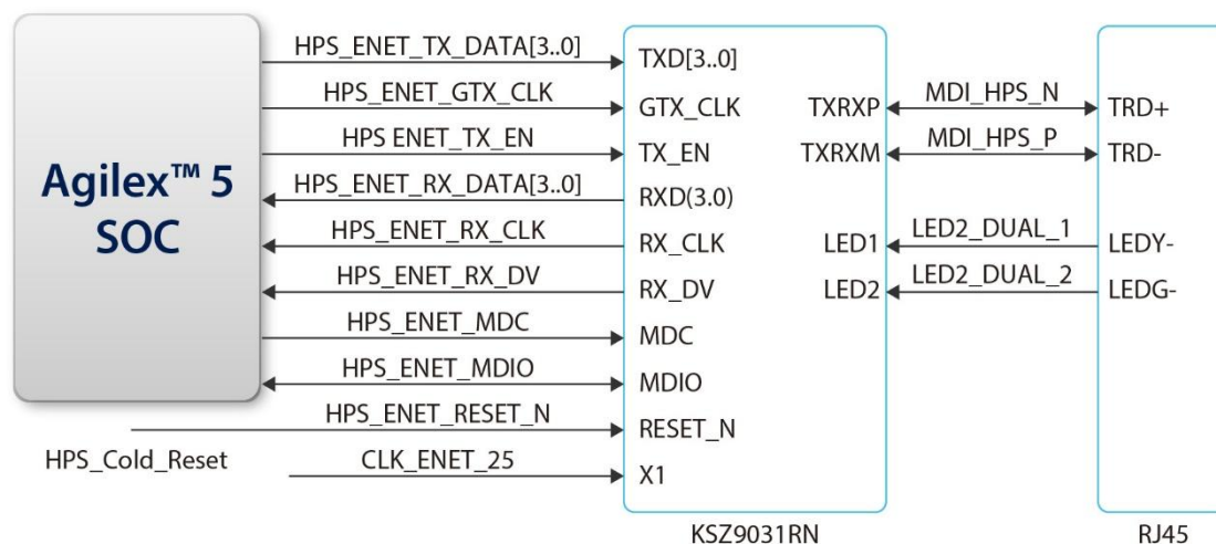
Figure 2-23 Connections between the HPS of Atum A5 and Ethernet PHY
