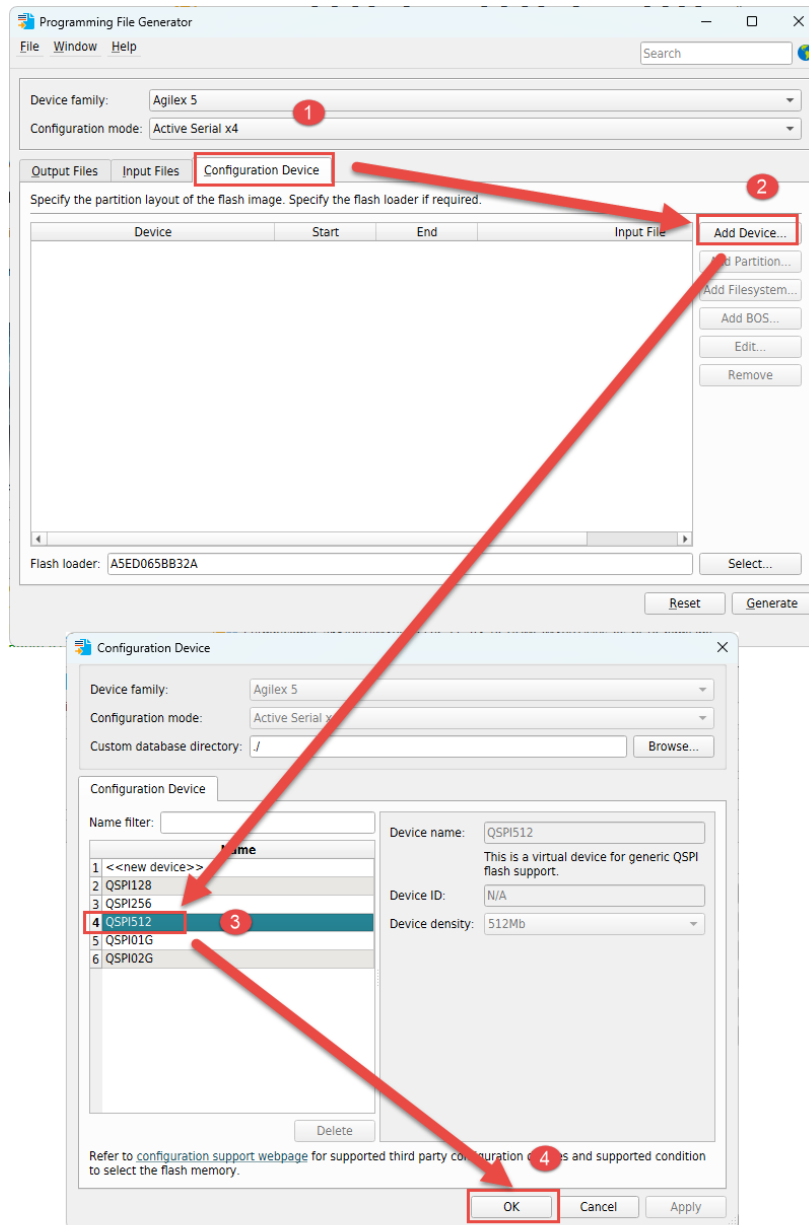
Figure 5-9 Setting Configuration Device
