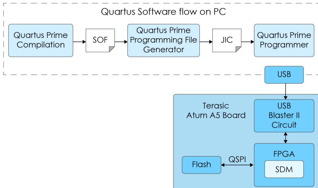
Figure 5-1 Programming Flow
