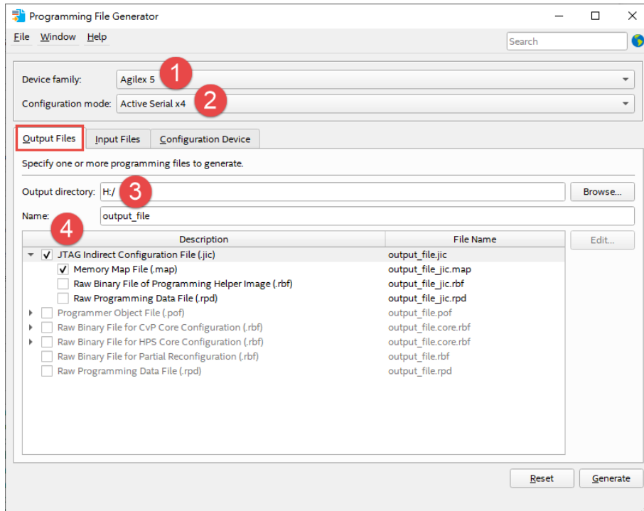
Figure 5-6 Setting output file
