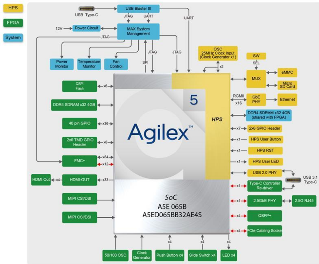
Figure 1-3 Block diagram of the Atum A5 board
