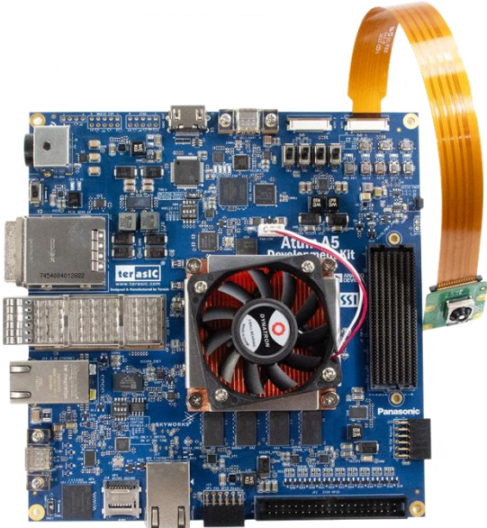
Figure 2-28 MIPI camera module connects to the board via cable
