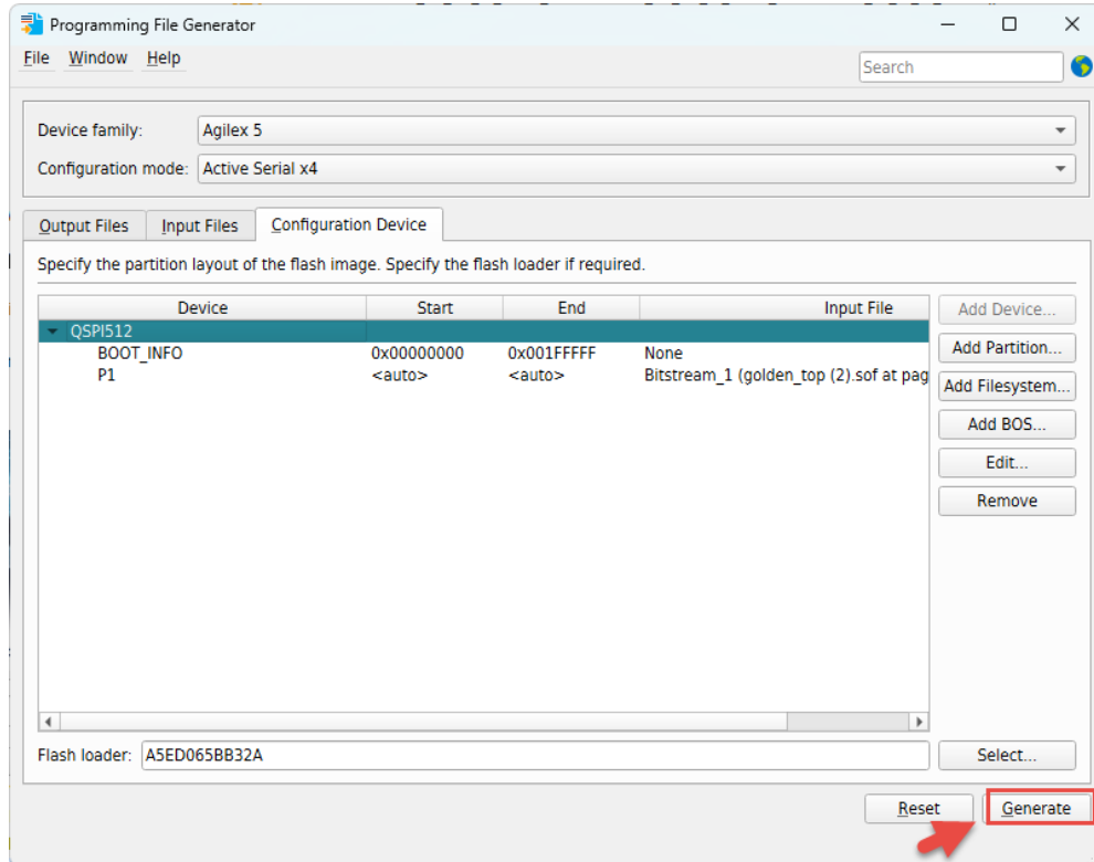
Figure 5-11 Generate .jic file
