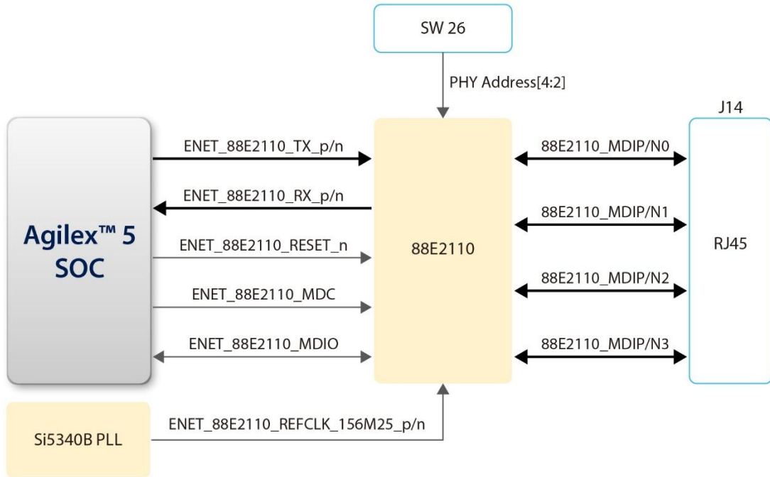
Figure 2-24 Connections between the FPGA and 88E2110 PHY
