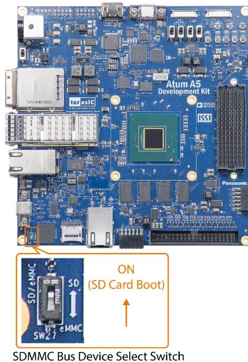
Figure 2-7 Position of slide switches SW27
