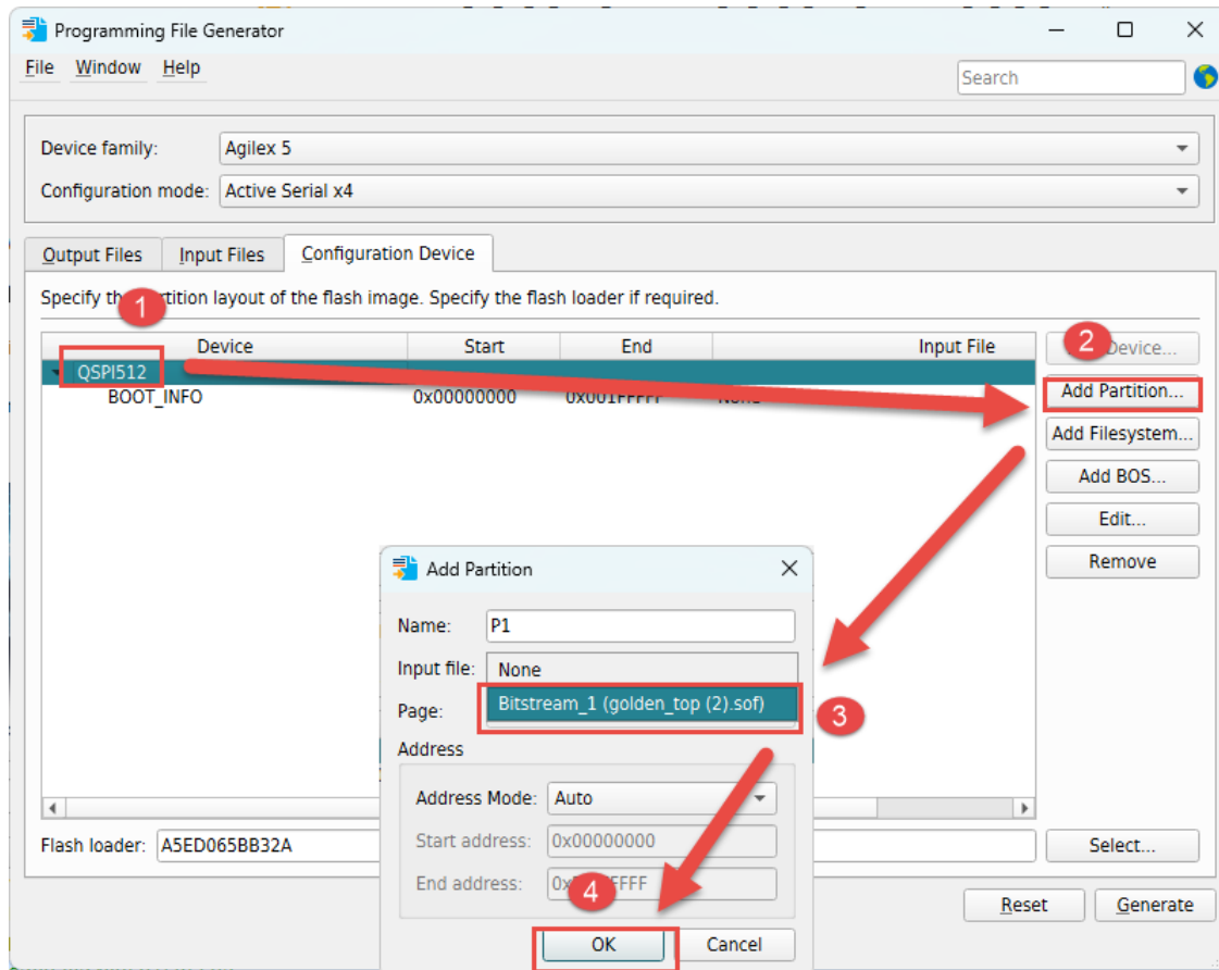
Figure 5-10 Setting Partition
