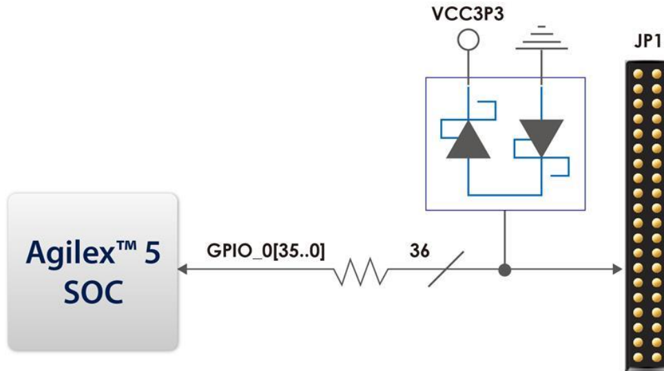
Figure 2-14 Connections between the GPIO header and Agilinx 5 SoC FPGA
