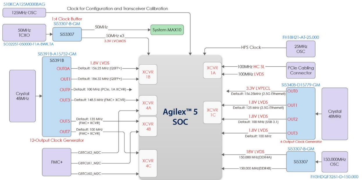
Figure 2-12 Clock circuit of the FPGA Board
