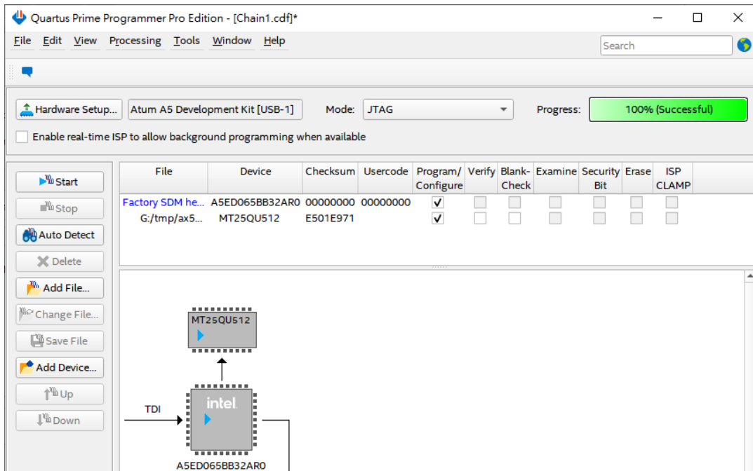
Figure 5-17 .jic file programmed successfully
