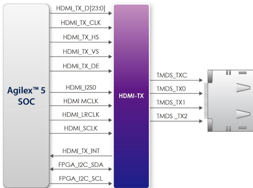
Figure 2-27 The HDMI output interface on the board
