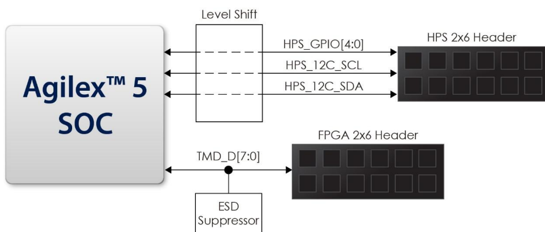
Figure 2-25 Connection between the 2x6 headers and FPGA
