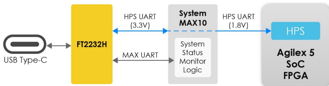
Figure 2-19 Three UART interface on the Atum A5 board
